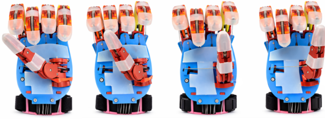
Fig. 5. Hand performing the Kapandji Test: touching the thumb to the tip of each of the four fingers.
