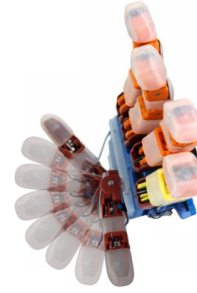
Fig. 7. Range of motion of the thumb with continuous opposition.
