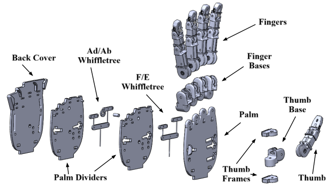
Fig. 2. Exploded view of underactuated hand mechanism. The hand consists of: i) four fingers with three pin joints each and springs for passive extension, ii) a thumb with two pin joints and springs for passive extension, iii) a thumb base and frames that enable the rotation, iv) the whiffletree controlling flexion/extension of all fingers, v) the whiffletree controlling adduction/abduction of the four fingers, and vi) the remaining components that make up the hand body and the palm.
