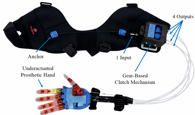
Fig. 1. The proposed anthropomorphic prosthetic hand integrates underactuated finger mechanisms with a body-powered actuation system. The design incorporates a gear-based selective clutch mechanism for mechanically switching between functional modes and internal differential mechanisms for compliant force distribution.
