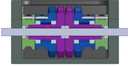
Fig. 3. Cross-sectional view of the gear-based clutch mechanism showing from left to right: Four finger Ad/Ab pulley (green), all finger F/E Gear and pulley (blue), four finger Ad/Ab gear (purple), neutral gear (purple), thumb opposition gear and pulley (blue), and neutral pulley (green).
