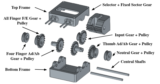
Fig. 4. Exploded view of the mode-switching transmission illustrating the top and bottom frames, selector with fixed sector gear, input gear–pulley assembly, output gear–pulley assemblies, and central shafts. The four finger Ad/Ab gear (left purple in Fig. 3) and pulley (left green in Fig. 3) are interconnected. Similarly, the neutral gear (right purple in Fig. 3) and pulley (right green in Fig. 3) are interconnected. The all finger F/E gear and pulley (left blue in Fig. 3) and the thumb opposition gear and pulley (right blue in Fig. 3) are designed as single parts.
