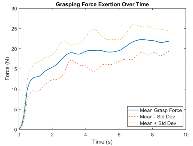
Fig. 10. Mean grasping force profile with \pm 1 standard deviation across ten power grasp trials. Peak mean force of 22.3 N was achieved at approximately t = 7.5 s, with a maximum single-trial force of 25.6 N.
